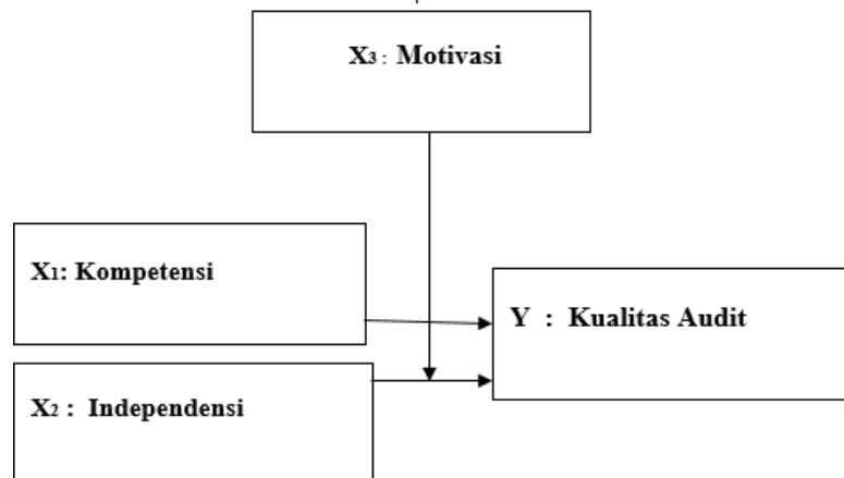
Gambar 1 Model Penelitian
